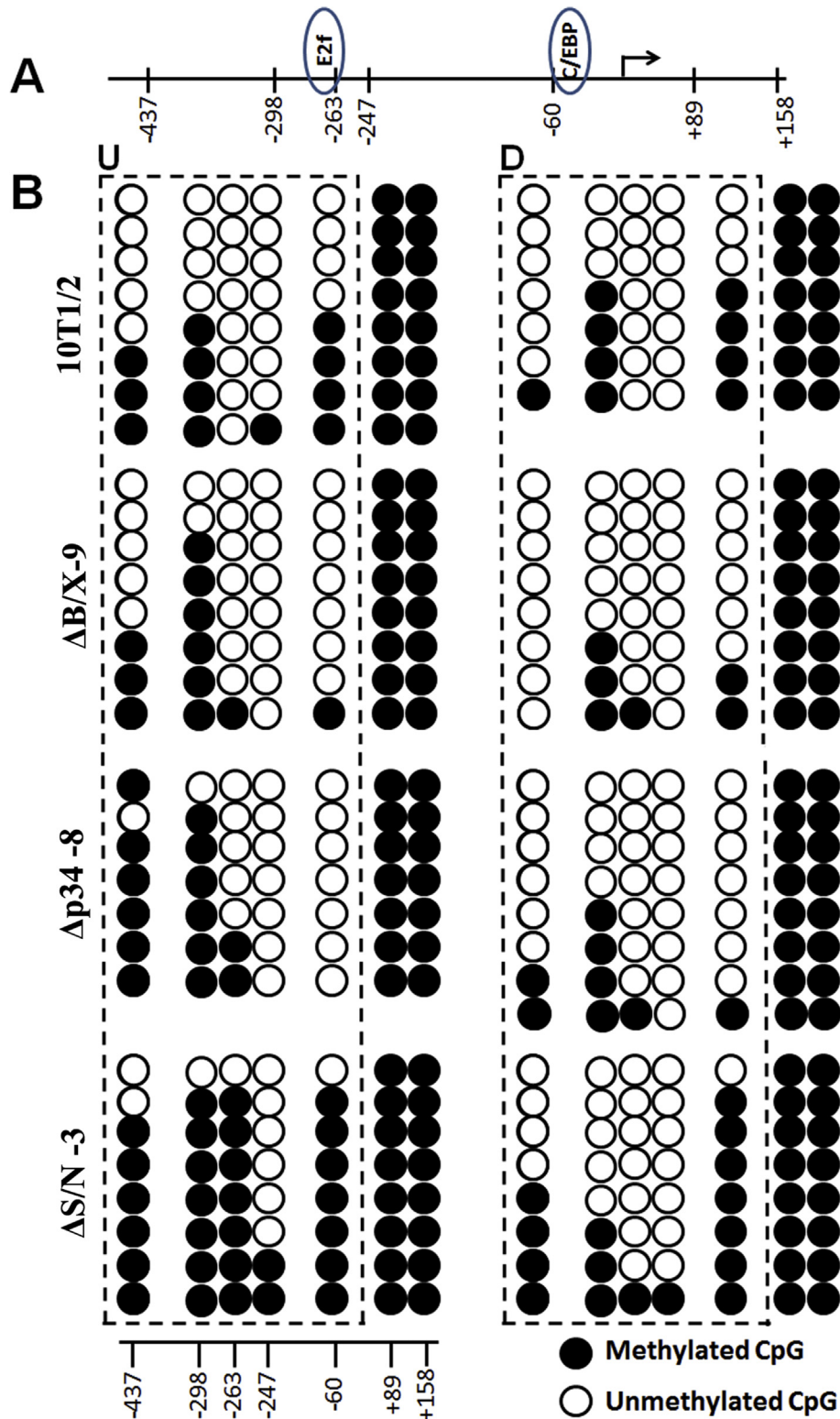
Figure 3 Promoter of the PPAR \gamma 2 is highly hypermethylated in undifferentiated \Delta S/N cells. (A) Schematic illustration of the PPAR \gamma 2 promoter. An arrow indicates the transcription start site (TSS) (+1 bp); short vertical lines indicate the positions of the CpG relative to the TSS. (B) Bisulfite sequencing analyses of the PPAR \gamma 2 promoter. Methylation status of the PPAR \gamma 2 in cells producing exogenous \Delta B/X, \Delta p34 or \Delta S/N was analyzed: (U) under undifferentiated conditions; (D) upon differentiation stimulus. The regions marked by dash lines represent the 5'upstream TSS region. At the bottom of the illustrations, the methylation status of the CpGs is shown.
