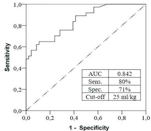
Fig. 7. Receiver operating characteristics curve of fluid balance POD-1 in acute kidney injury (AKI) and non-AKI patients.
