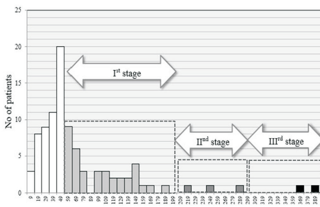
Fig. 3. \Delta SCr (serum creatinine) histogram.
